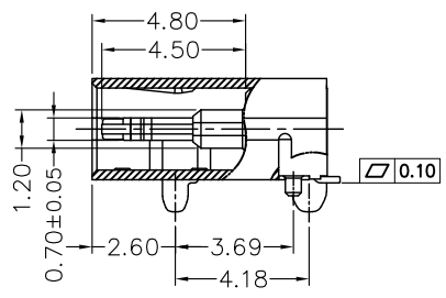
CUTAWAY
