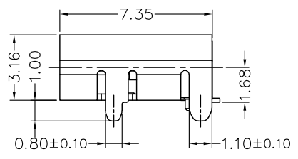
CUTAWAY
