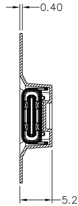
Cutaway-Y
